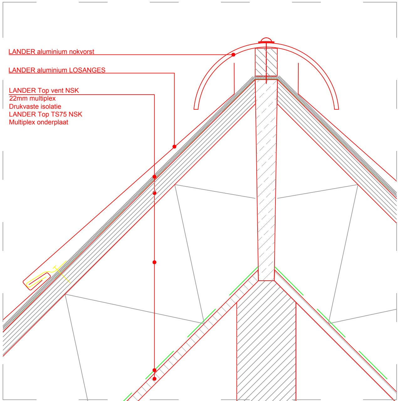
Gootdetail V-01m
