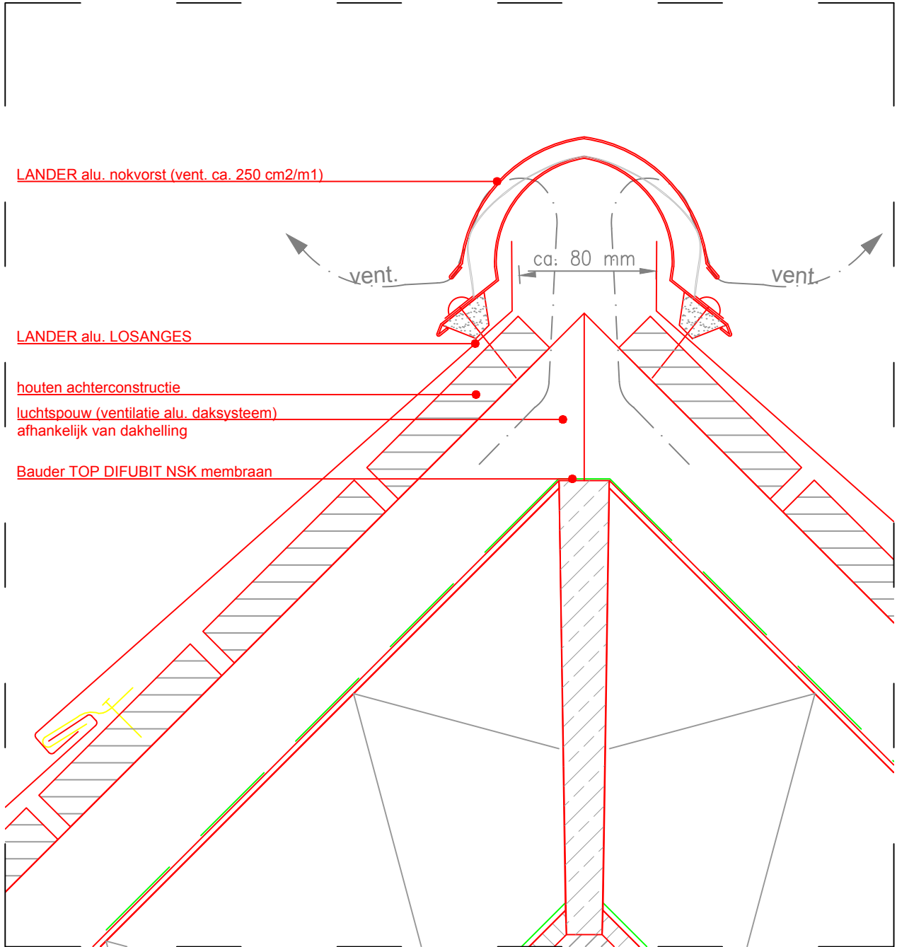
Nokdetail V-02
