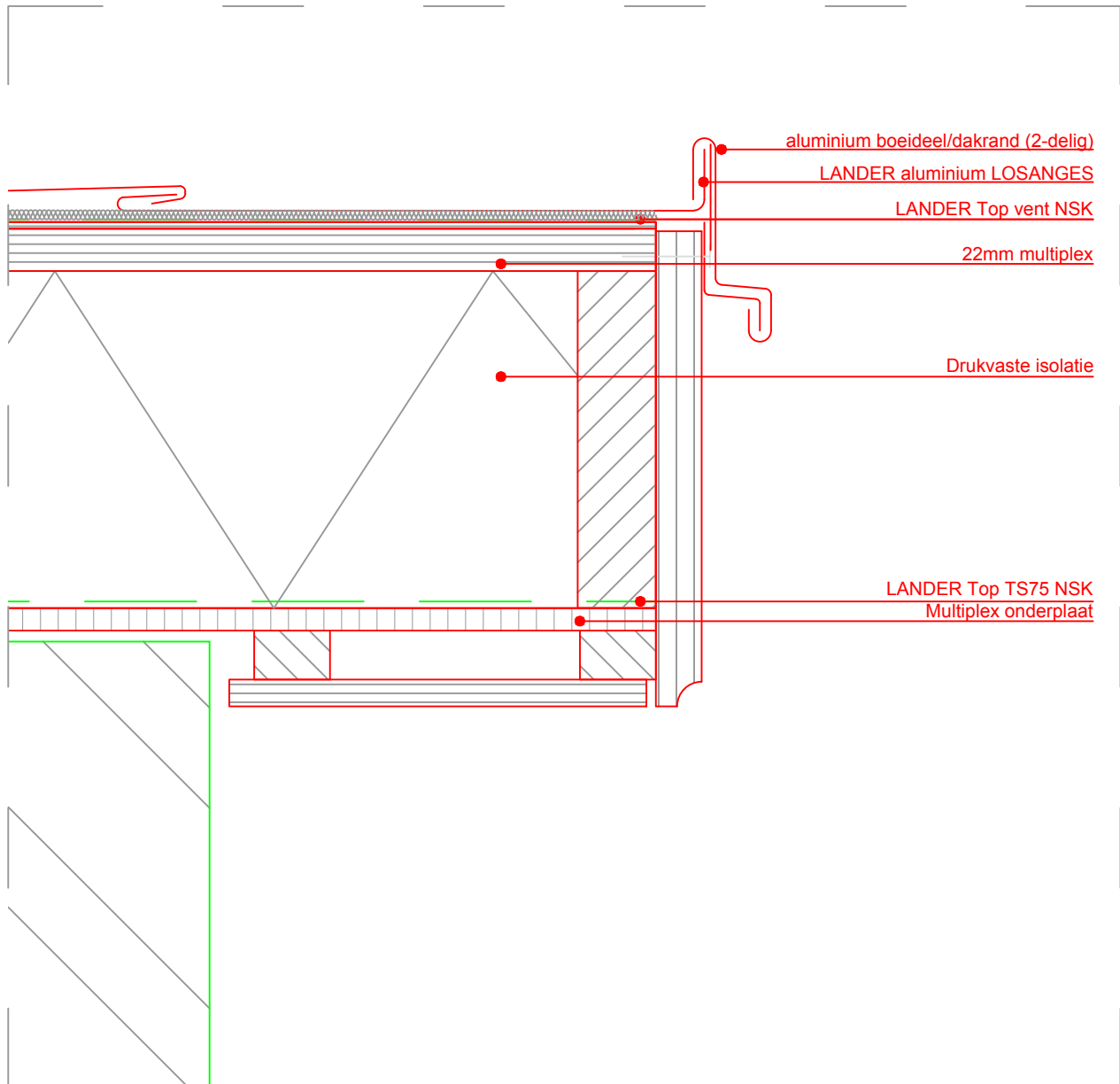
Gootdetail H-03m(a)
