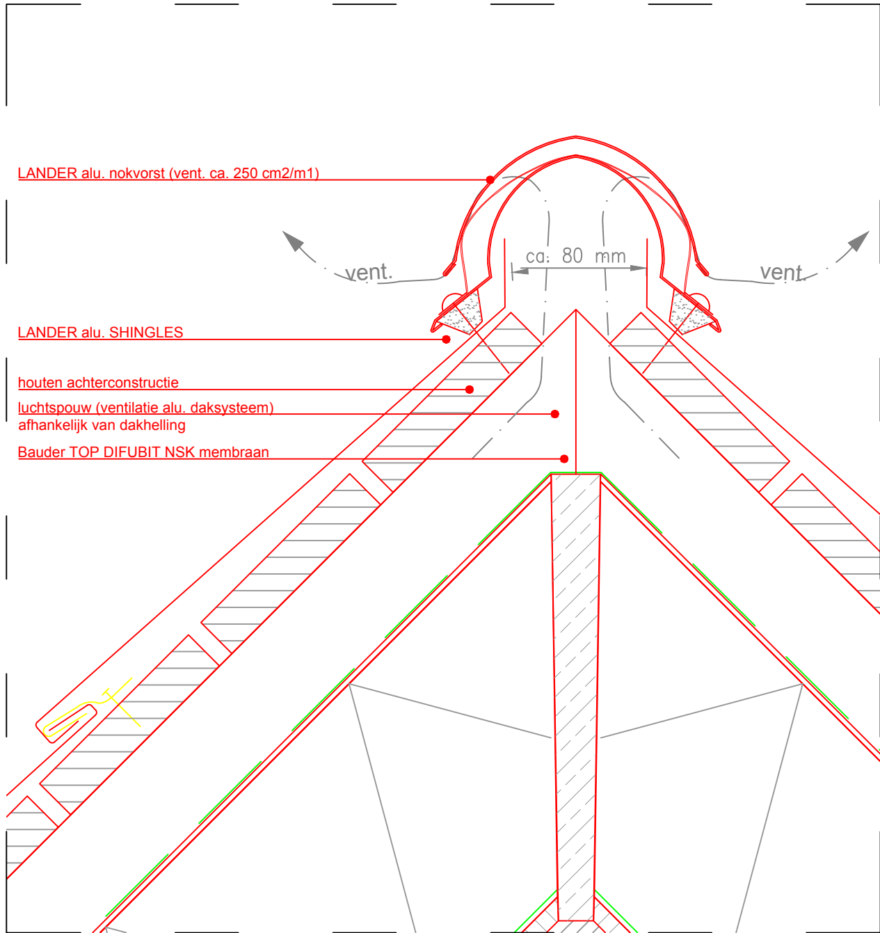
Nokdetail V-02
