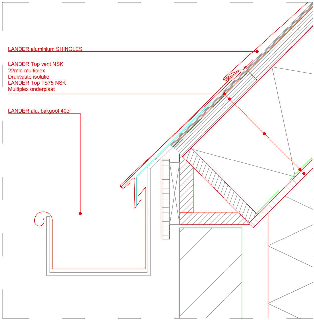
Gootdetail V-01m
