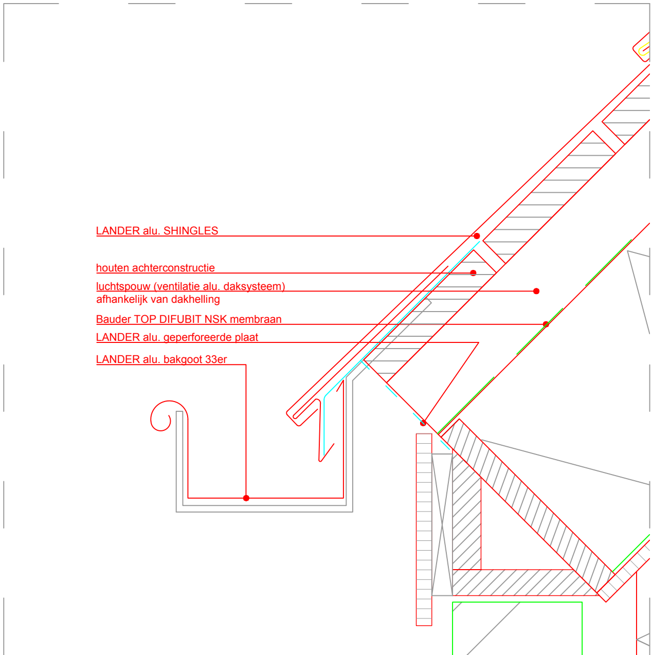
Gootdetail V-01
