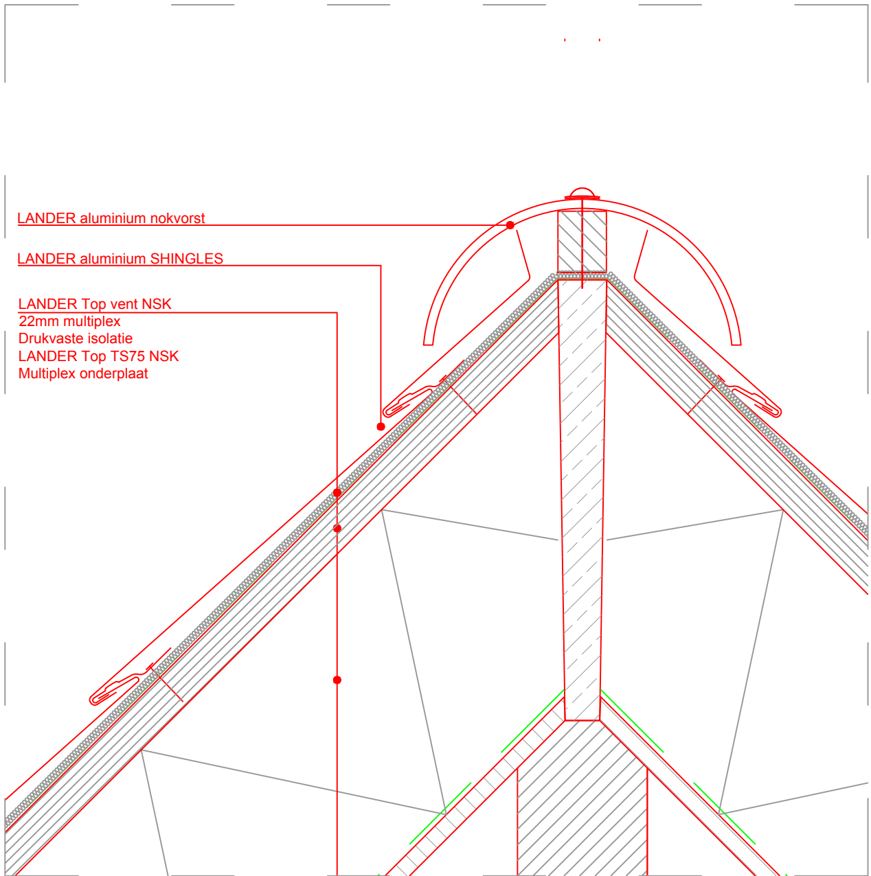
Nokdetail V-02m
